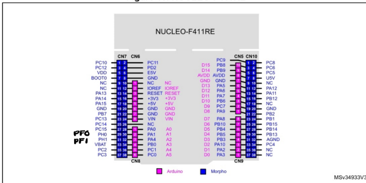
Figure 18. NUCLEO-F411RE
